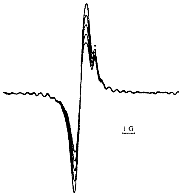
Fig. 1. ESR spectra of the fullereryl radical in a saturated toluene solution of C_{60} containing 10^{-2} mol L^{-1} of dimer 1 at 300 K recorded after 132 s. The signal from defects of the quartz Dewar tube is marked by the asterisk.
