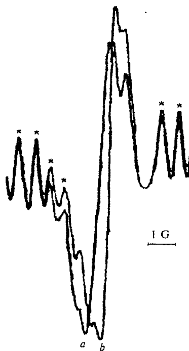
Fig. 2. ESR spectra of the metal-containing fullerenyl radical in mesitylene at 300 K ( a ) and demetallated fullerenyl radical during heating at 370 K for 6 min ( b ). The components of the ESR-spectrum of radical 2 are marked by the asterisks.
